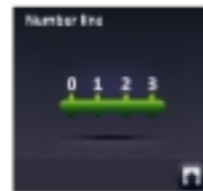
Numberline
